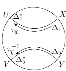
Figure 1 \Delta_1 and \Delta_2 satisfy the condition (3.2).
