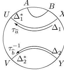
Figure 3 The axis c_g \subset \Delta_1^* \subset \Delta_2 .
