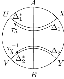
Figure 2 The axis c_g crosses both \partial\Delta_1 and \partial\Delta_2 .
