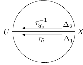
Figure 9 The axis c_g = \partial\Delta_1 = \partial\Delta_2 .
