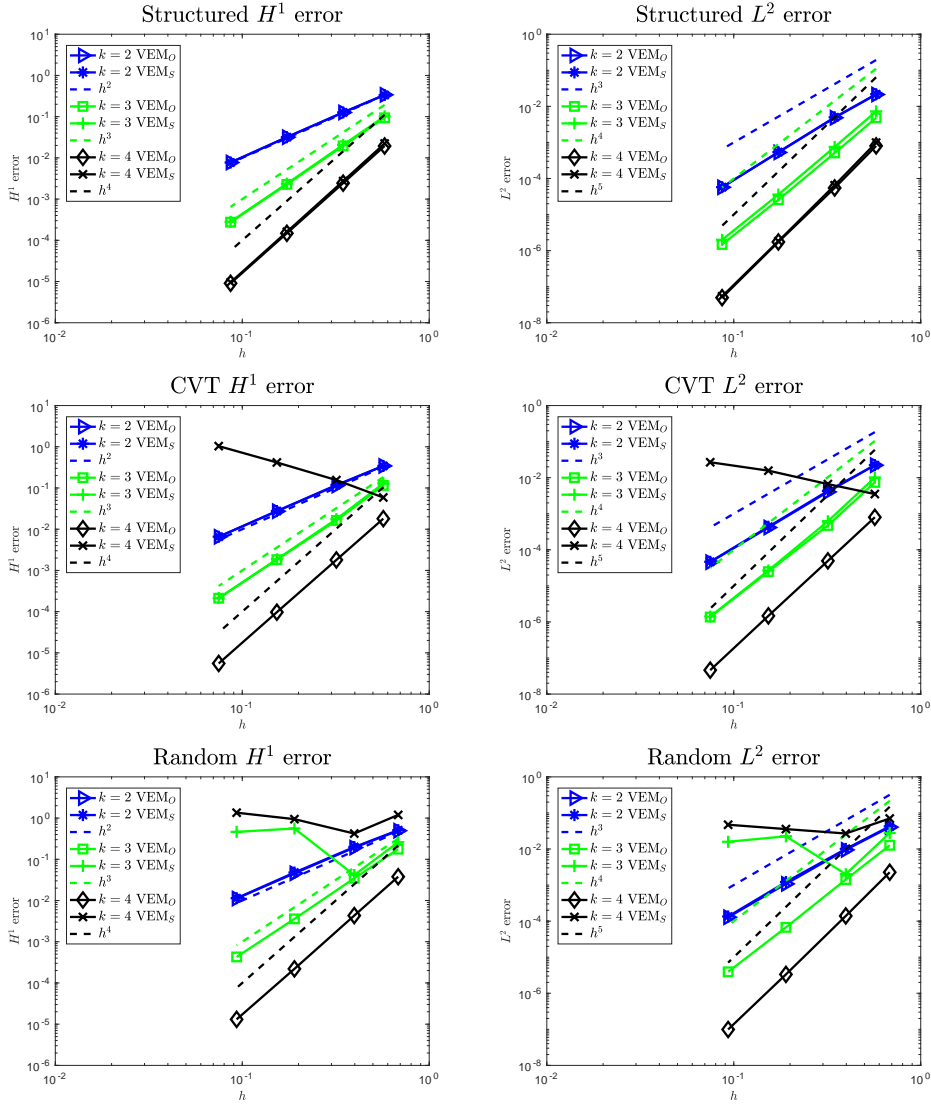
Figure 4 Test case 2: Comparison between \text{VEM}_O and \text{VEM}_S for all meshes.
