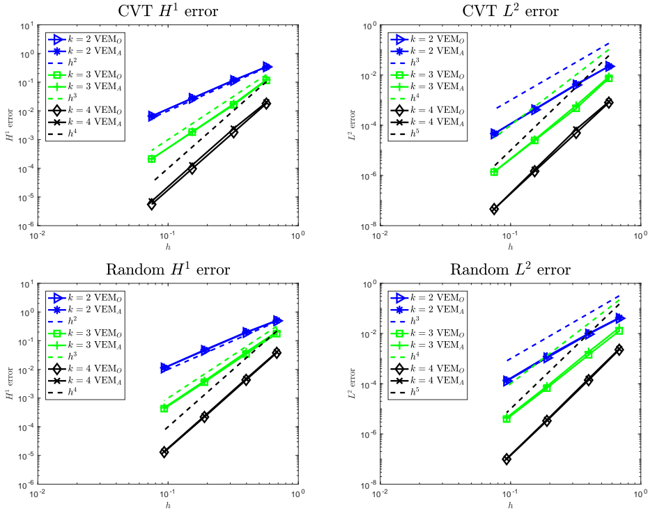
Figure 5 Test case 3: Comparison between \text{VEM}_O and \text{VEM}_A for CVT and Random meshes.
